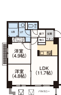
●2LDK / 47.96㎡
