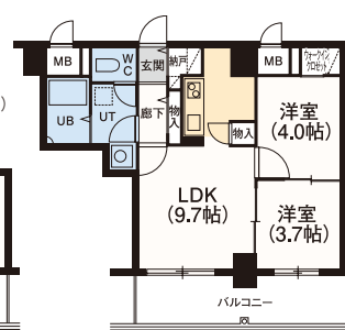
●2LDK / 40.44㎡
